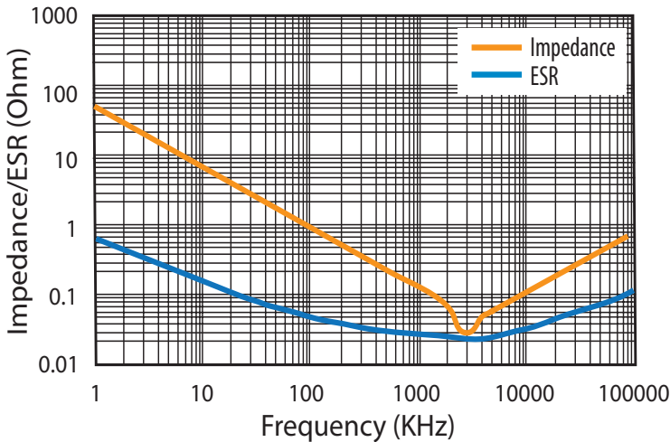
1. Impedance/ESR vs. Frequency
