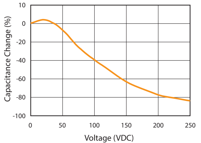
2. Capacitance vs. DC Voltage
