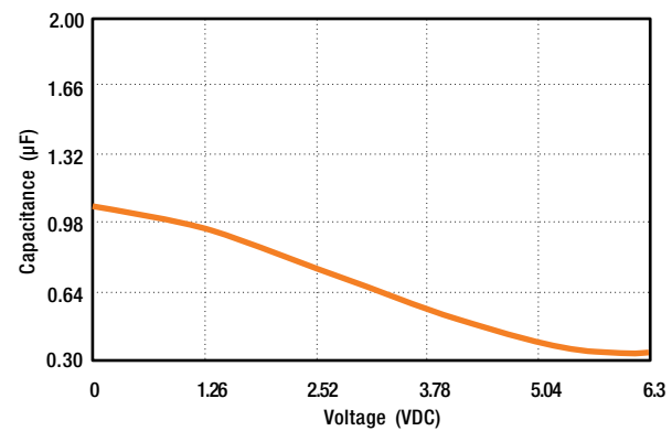
2. Capacitance vs. DC Voltage
