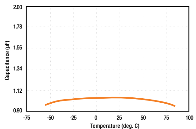
4. Capacitance vs. Temperature
