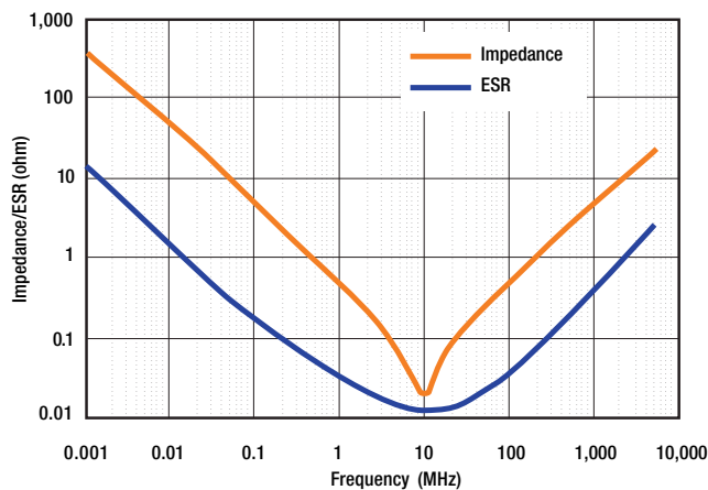
1. Impedance /ESR vs. Frequency
