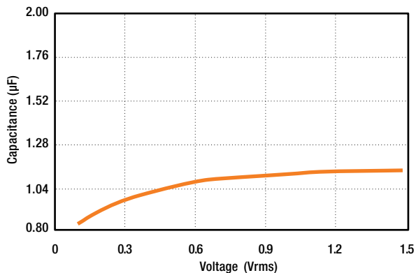
3. Capacitance vs. AC Voltage
