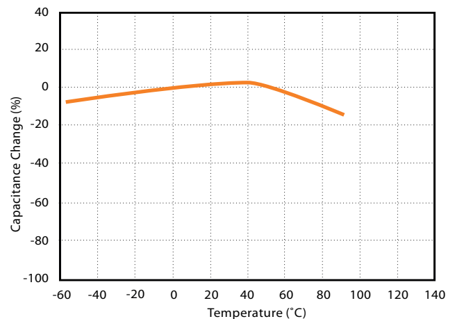
4. Capacitance - Temperature Characteristics
