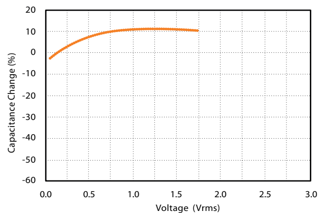
3. Capacitance - AC Voltage Characteristics
