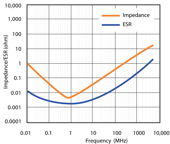
1. Impedance /ESR - Frequency
