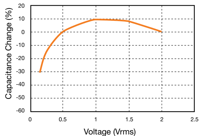
3. Capacitance vs. AC Voltage
