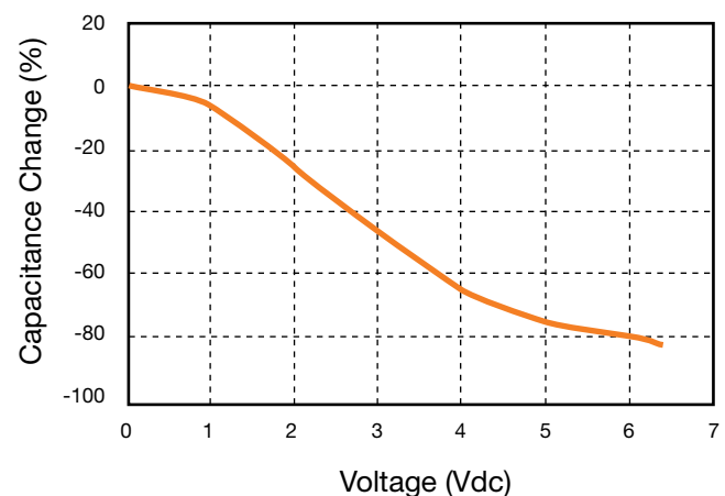
2. Capacitance vs. DC Voltage
